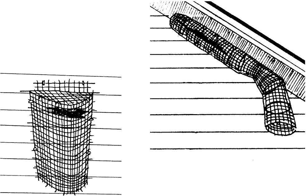
Figure 5. Inexpensive, one-way bat exclusions can be made with wire screen. Bats can exit through the open bottom, but cannot fly up to return. Standard design, left, is ideal for holes and small gaps in siding, but can be modified, right, to cover long cracks or gaps along eaves or between siding and a chimney.
